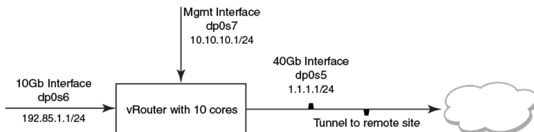
Figure 2. Controlling IPsec crypto cores
