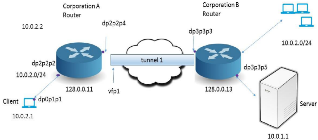
Figure 9. VFP Interface for an IPsec VPN
