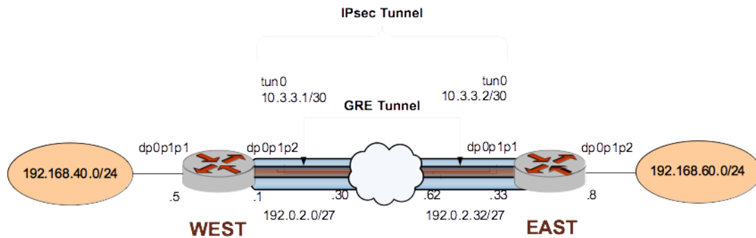
Figure 6. GRE tunnel protected by an IPsec tunnel
