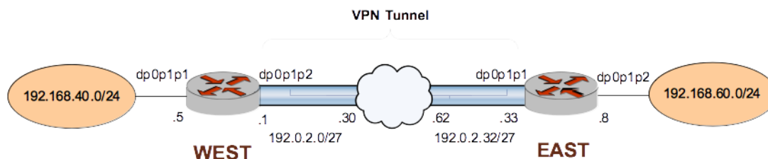
Figure 3. Basic site-to-site IPsec VPN connection
