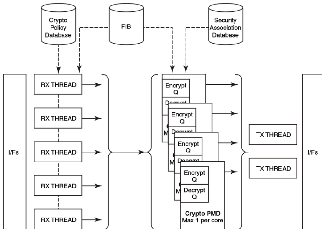
Figure 1. Multiple crypto engines overview
