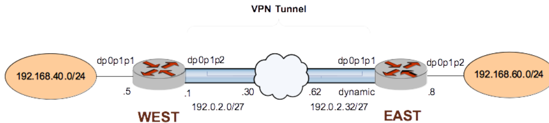
Figure 4. IPsec VPN connection with dynamic IP address
