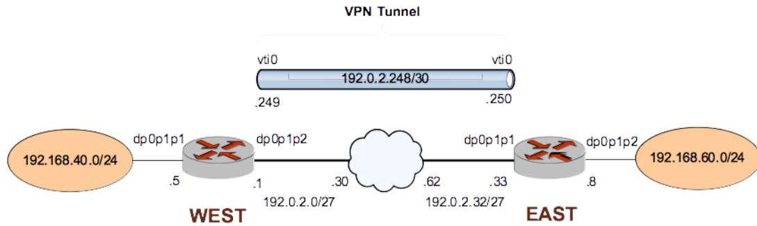
Figure 7. IPsec VPN connection with virtual tunnel interfaces
