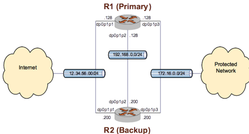
Figure 4. Configuration synchronization
