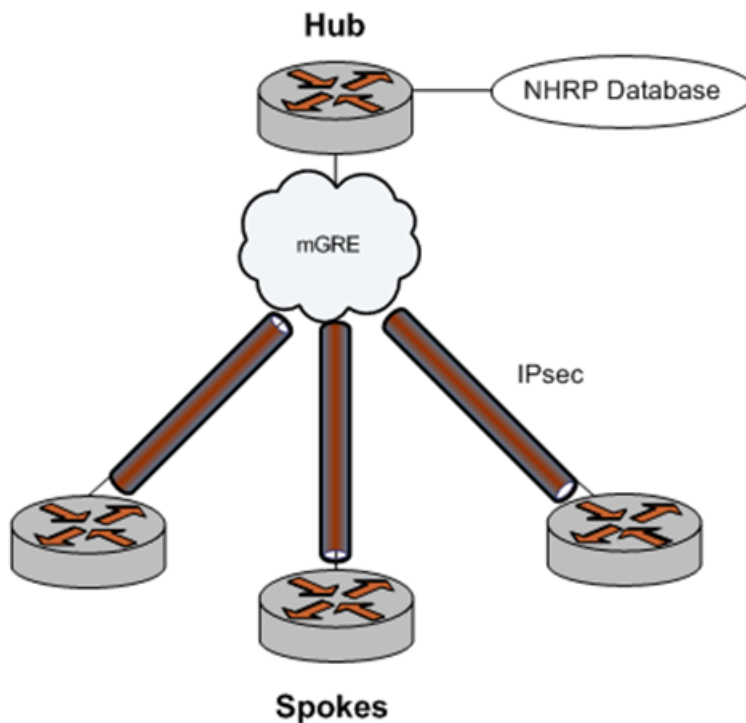
Figure 1. IPsec
