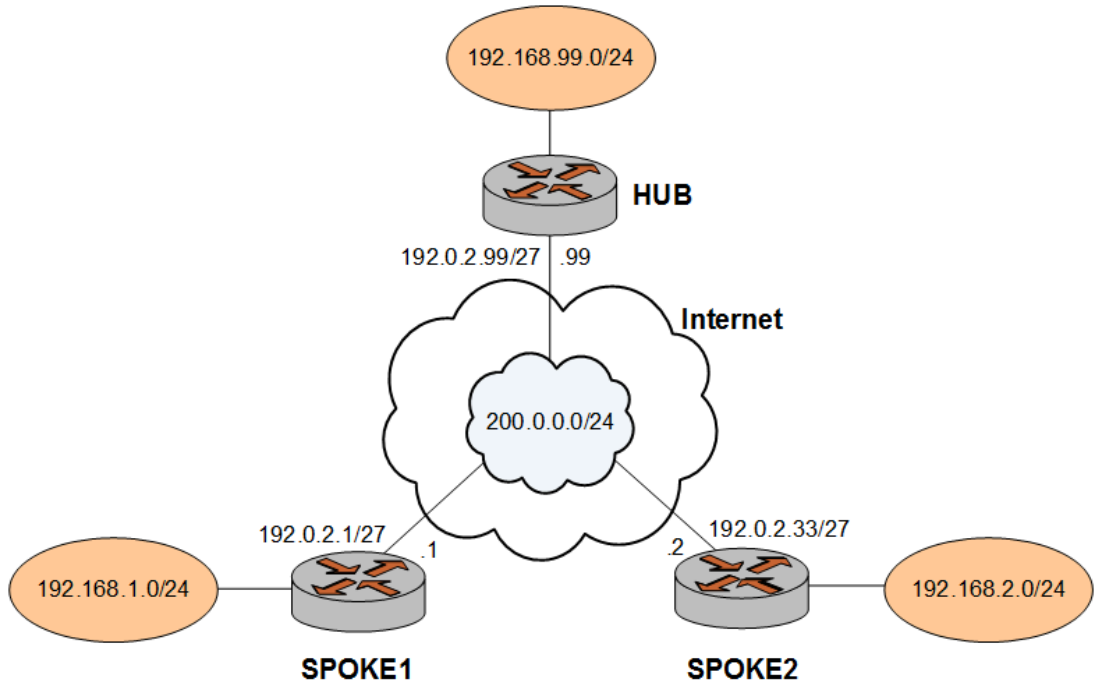
Figure 2. Basic mGRE tunnel network
